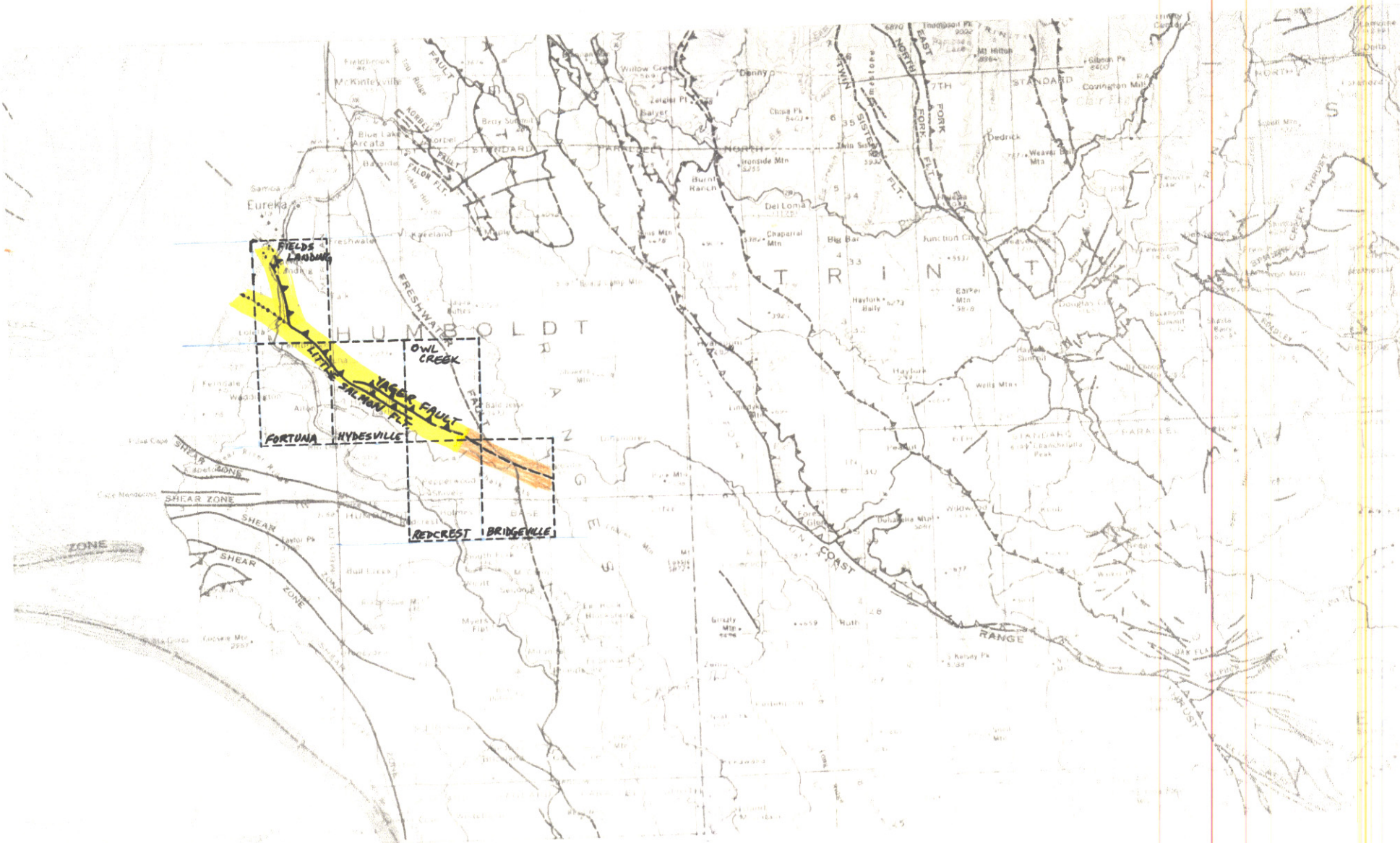
FER-142. Figure 1. Location of the Little Salmon and Yager faults. Yellow from Jennings (1975, unmodified); orange from Kelsey and Allwardt (1974).
